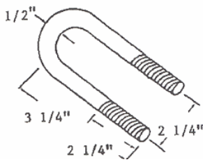
TRAINLINE 'U' BOLT
