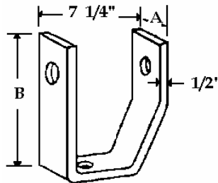
TRAINLINE BRACKET STRAP
