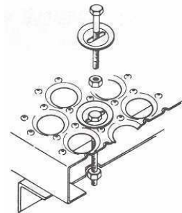
Bolt Seats – Part #4029 Round Hole Grating
