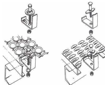
J Clips for Round Hole & Diamond Hole Grating
