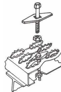
Bolt Seats – Part #B&B-BS Diamond Hole Grating
