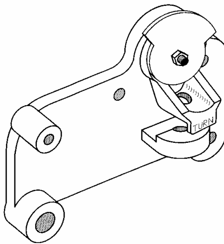
SLIDING DOOR LOCK PLATE ASSEMBLY Part # 6019
