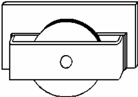
DOOR ROLLER CONVERSION KIT Part # 6008 – 8-3/4" Wide
