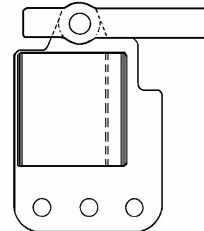
HOLD OPEN ASSEMBLY Part # 6045-LH OPPOSITE HAND Part # 6045-RH AS SHOWN
